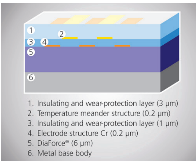
Schematic representation of the thin-film system.
